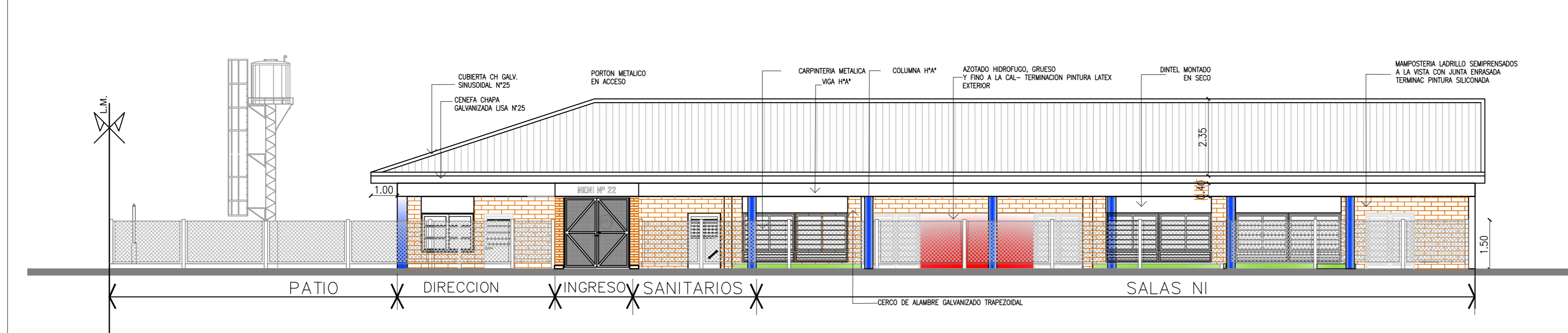
FACHADACALLE CLORINDA Esc 1:100
